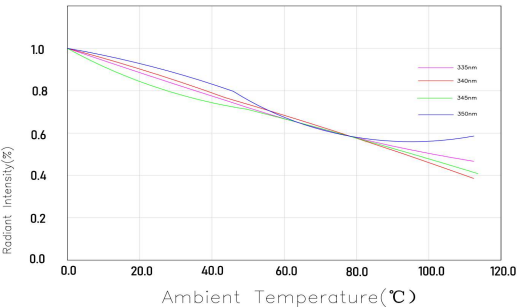
(4) 辐射强度VS温度 Radiant Intensity VS Ambient Temperature
