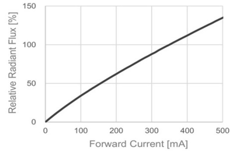
(3) 辐射强度VS电流 Radiated power VS current
