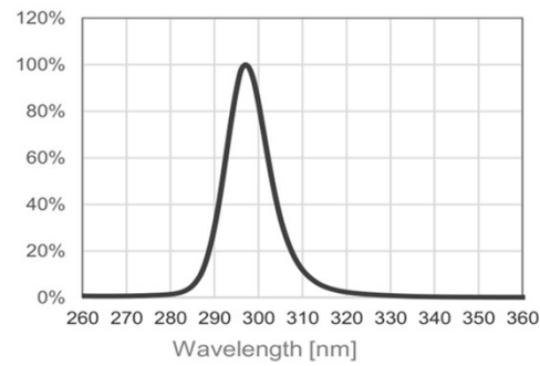
(1) 相对光谱分布Relative spectral distribution
