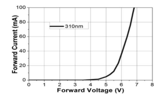
(2) I-V特性 I-V Characteristic
