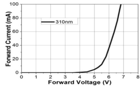
(2) I-V特性 I-V Characteristic
